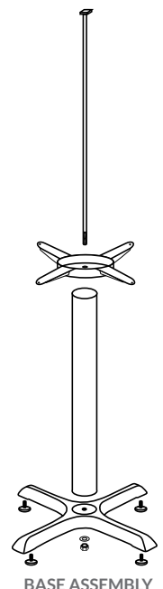
BASE ASSEMBLY
